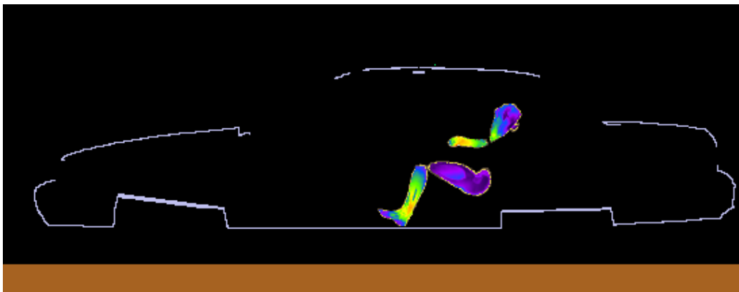
Figure 6. SAR distribution at 167.7 MHz in the passenger model produced by the roof-mount HAD4009A antenna. The contour plot is relative to the plane where the peak 1-g average SAR for this exposure condition occurs.
