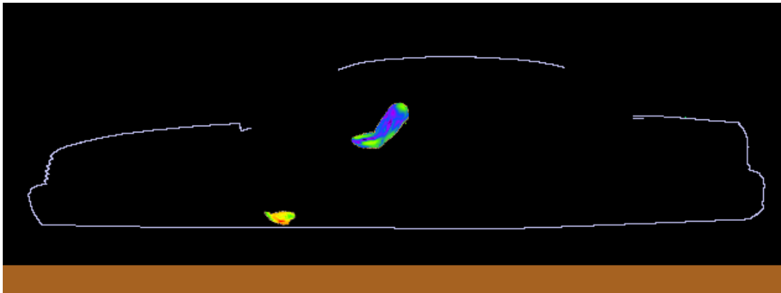
Figure 4. SAR distribution at 498.0000 MHz in the driver model produced by the trunk mount HAED4004A antenna. The contour plot is relative to the plane where the peak 1-g average SAR for this exposure condition occurs.
