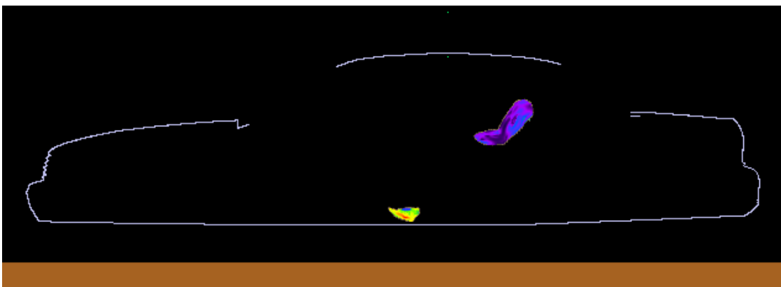
Figure 7. SAR distribution at 445.0125 MHz in the passenger model produced by the roof-mount HAE4011A antenna. The contour plot is relative to the plane where the peak 1-g average SAR for this exposure condition occurs.
