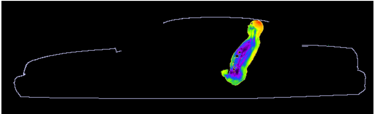
Figure 3. SAR distribution at 484.0000 MHz in the passenger back side model produced by the trunk mount HAD4004A antenna. The contour plot is relative to the plane where the peak 1-g average SAR for this exposure condition occurs.
