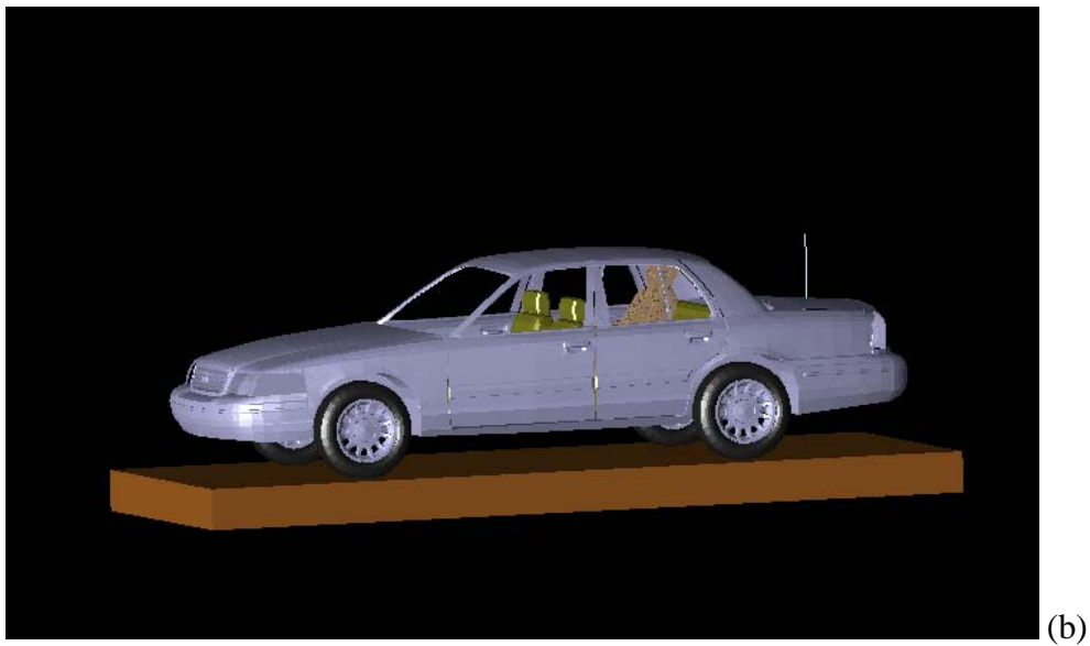
Figure 3: Passenger model exposed to roof mounted (a) and trunk-mounted (b) antennas: XFDTD geometry.
