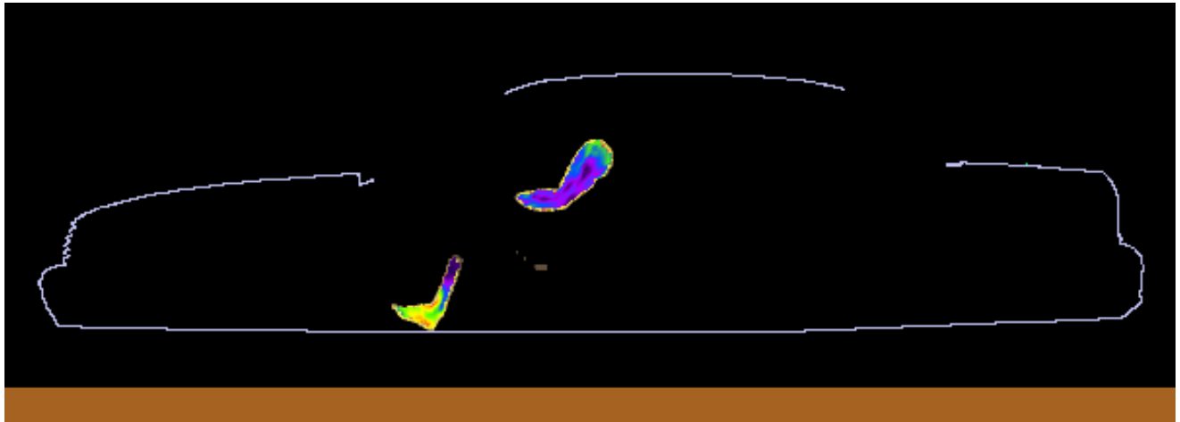
Figure 4. SAR distribution at 450.0000 MHz in the driver model produced by the trunk mount HAD4003A antenna. The contour plot is relative to the plane where the peak 1-g average SAR for this exposure condition occurs.
