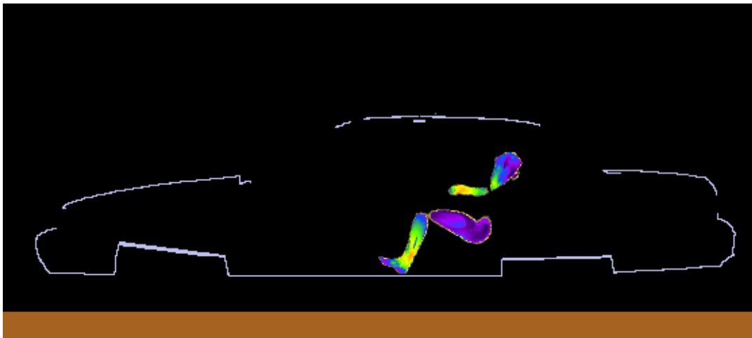
Figure 6. SAR distribution at 167.7 MHz in the passenger back side model produced by the roof-mount HAD4009A antenna. The contour plot is relative to the plane where the peak 1-g average SAR for this exposure condition occurs.
