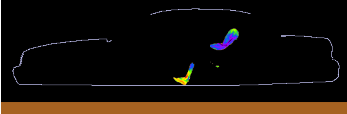
Figure 7. SAR distribution at 457.5000 MHz in the passenger model produced by the roof-mount HAE4011A antenna. The contour plot is relative to the plane where the peak 1-g average SAR for this exposure condition occurs.
