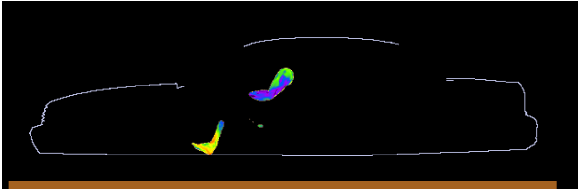
Figure 4. SAR distribution at 406.5 MHz in the driver model produced by the trunk mount HAD6012A antenna. The contour plot is relative to the plane where the peak 1-g average SAR for this exposure condition occurs.
