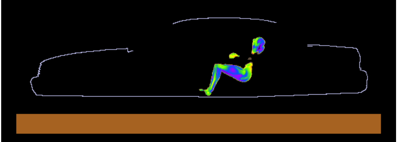
Figure 5. SAR distribution at 419.5 MHz in the passenger model produced by the roof-mount HAE6012A antenna. The contour plot is relative to the plane where the peak 1-g average SAR for this exposure condition occurs.
