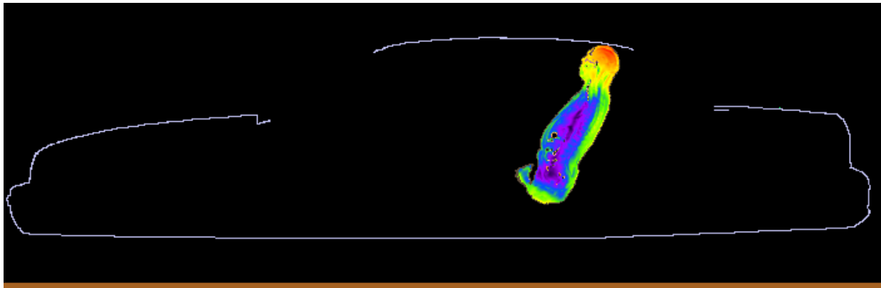
Figure 3. SAR distribution at 406.5 MHz in the passenger back side model produced by the trunk mount HAE6012A antenna. The contour plot is relative to the plane where the peak 1-g average SAR for this exposure condition occurs.
