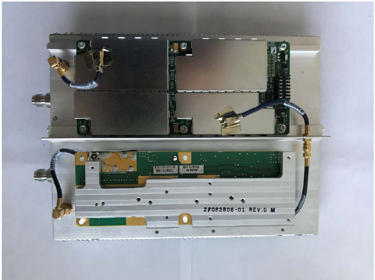
Finger stock was added on both long partition edges.
