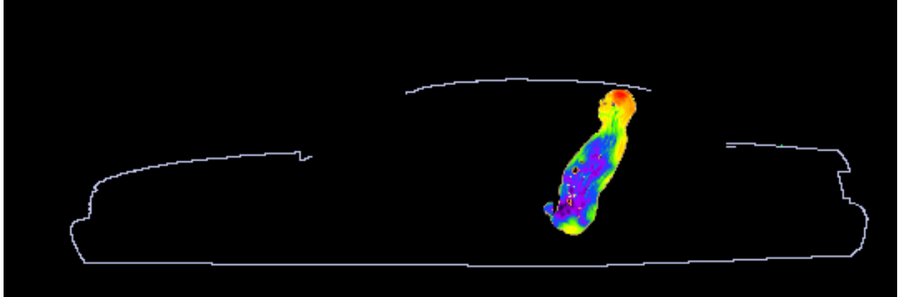
Figure 3. SAR distribution at 806 MHz in the passenger back center model produced by the trunk mount HAF4016A antenna. The contour plot is relative to the plane where the peak 1-g average SAR for this exposure condition occurs.
