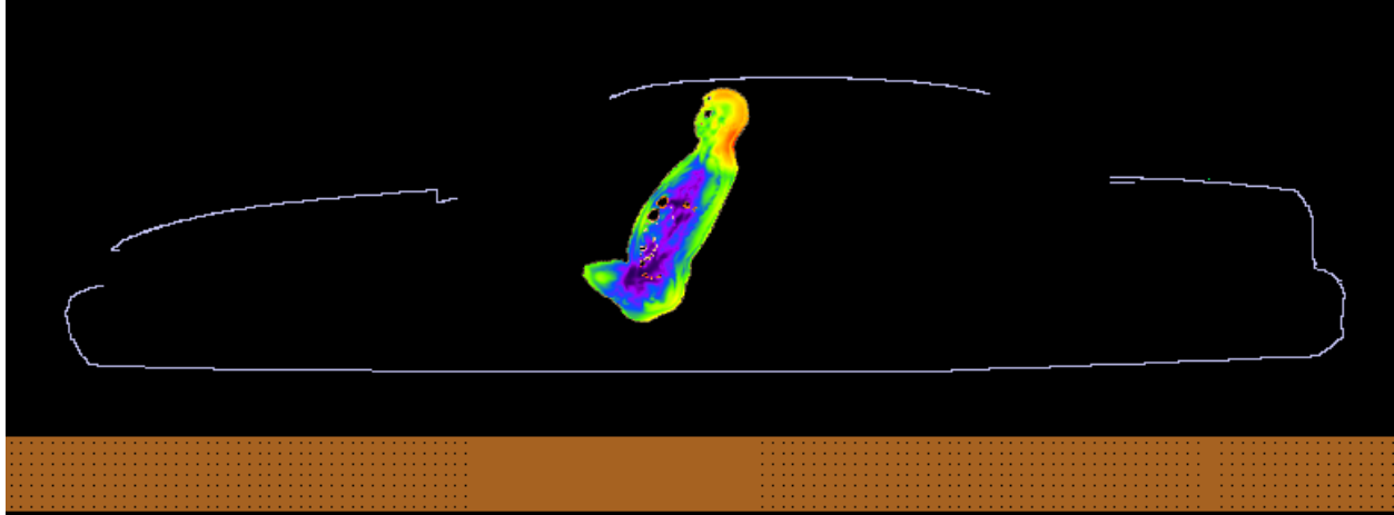
Figure 3. SAR distribution at 869.0 MHz in the driver model produced by the roof-mount HAF4016A antenna. The contour plot is relative to the plane where the peak 1-g average SAR for this exposure condition occurs.
