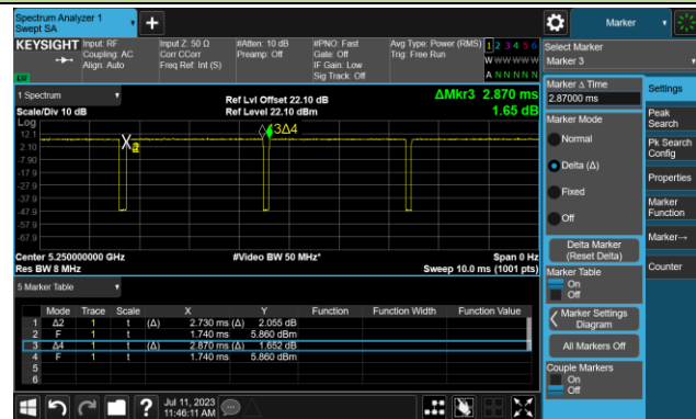
802.11ax-HE40 (T = 5.340ms)
