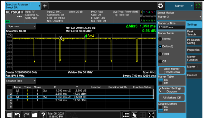
802.11ac-VHT20 (T = 1.311ms)
