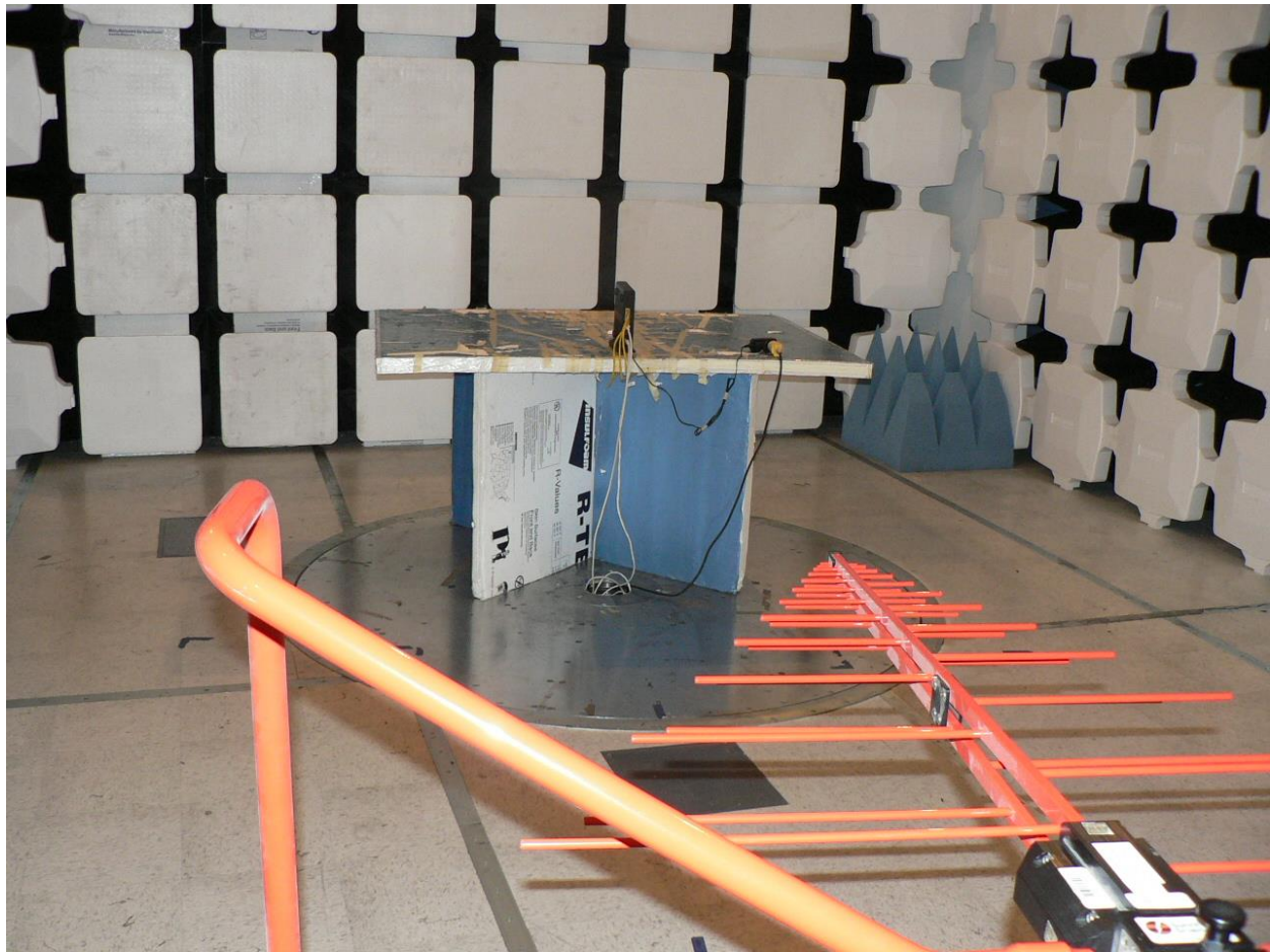
Digital Emissions (0.03-1 GHz) Front View
