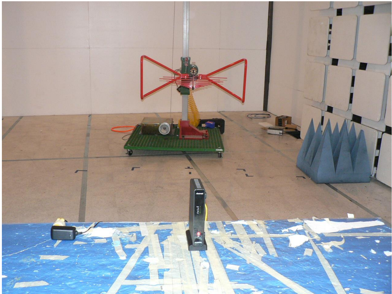
Digital Emissions (0.03-1 GHz) Rear View
