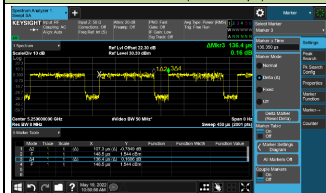
802.11ac-VHT160 (T = 107.3μs)
