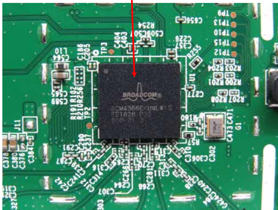
5G WIFI RF Chip IC – Top View
