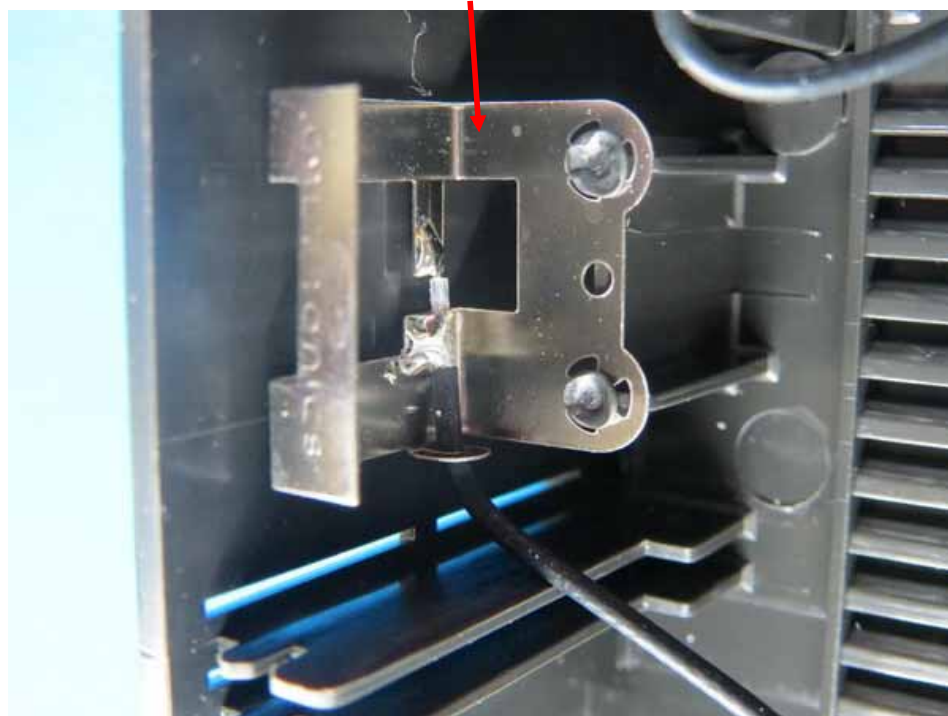
2.4G WIFI Antenna 1 – Top View
