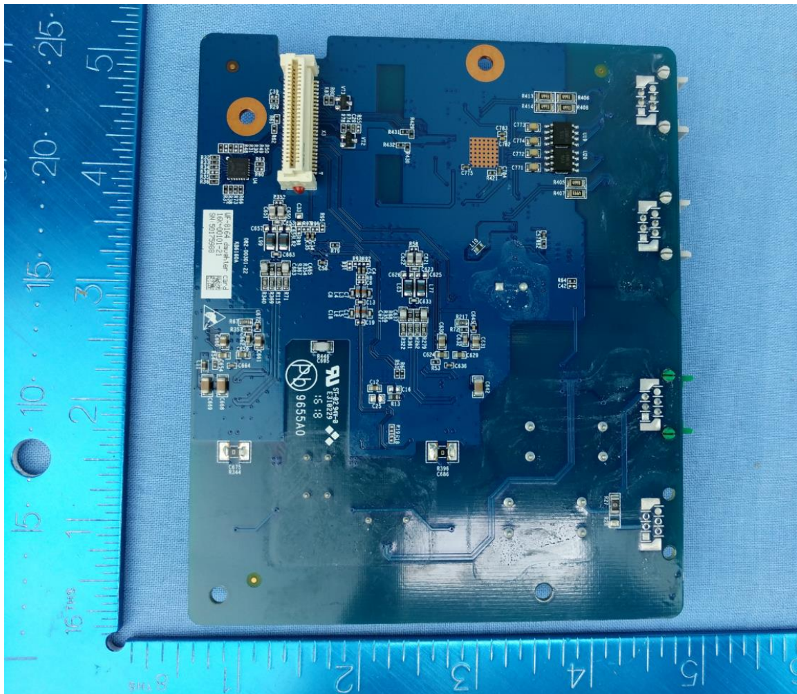
Modem Board Bottom View
