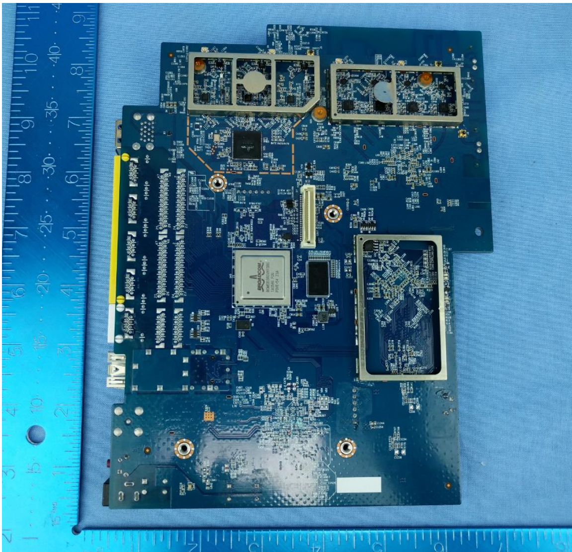
Main Board Bottom View - no shielding
