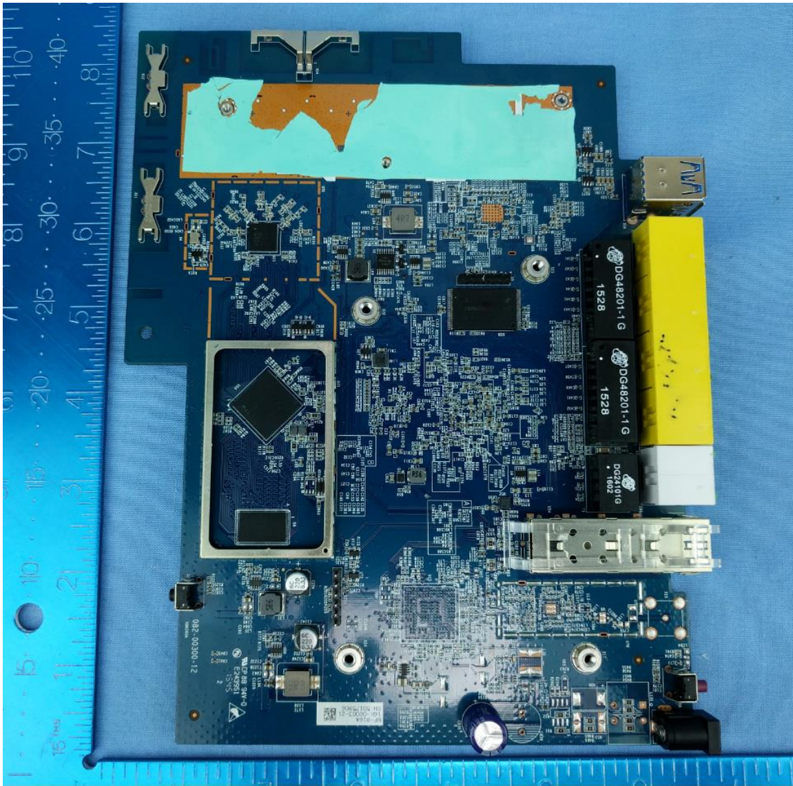
Main Board Top View – no shielding
