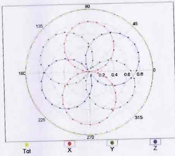
f=600 MHz,TEM
