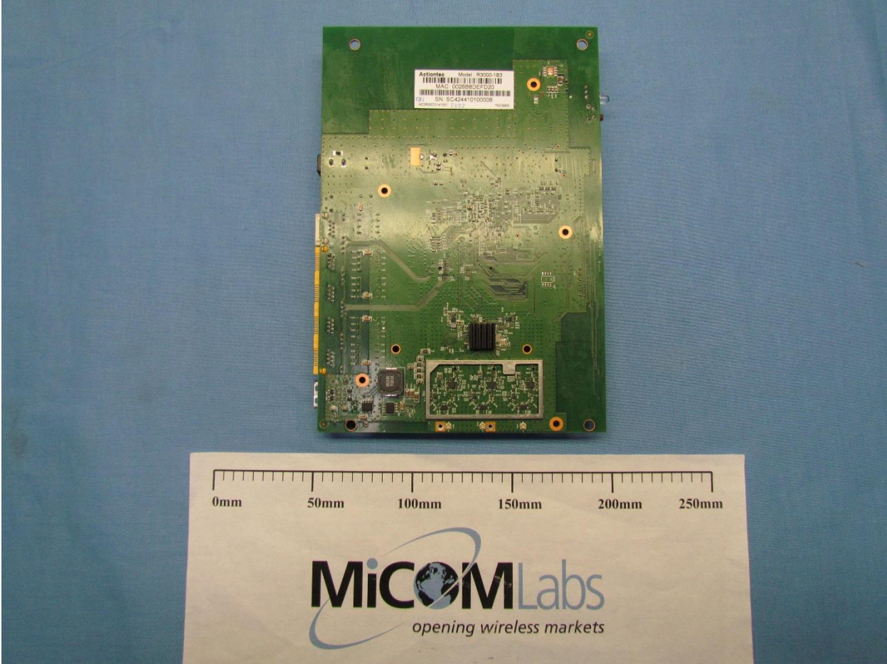
EUT Back with radio card shield off
