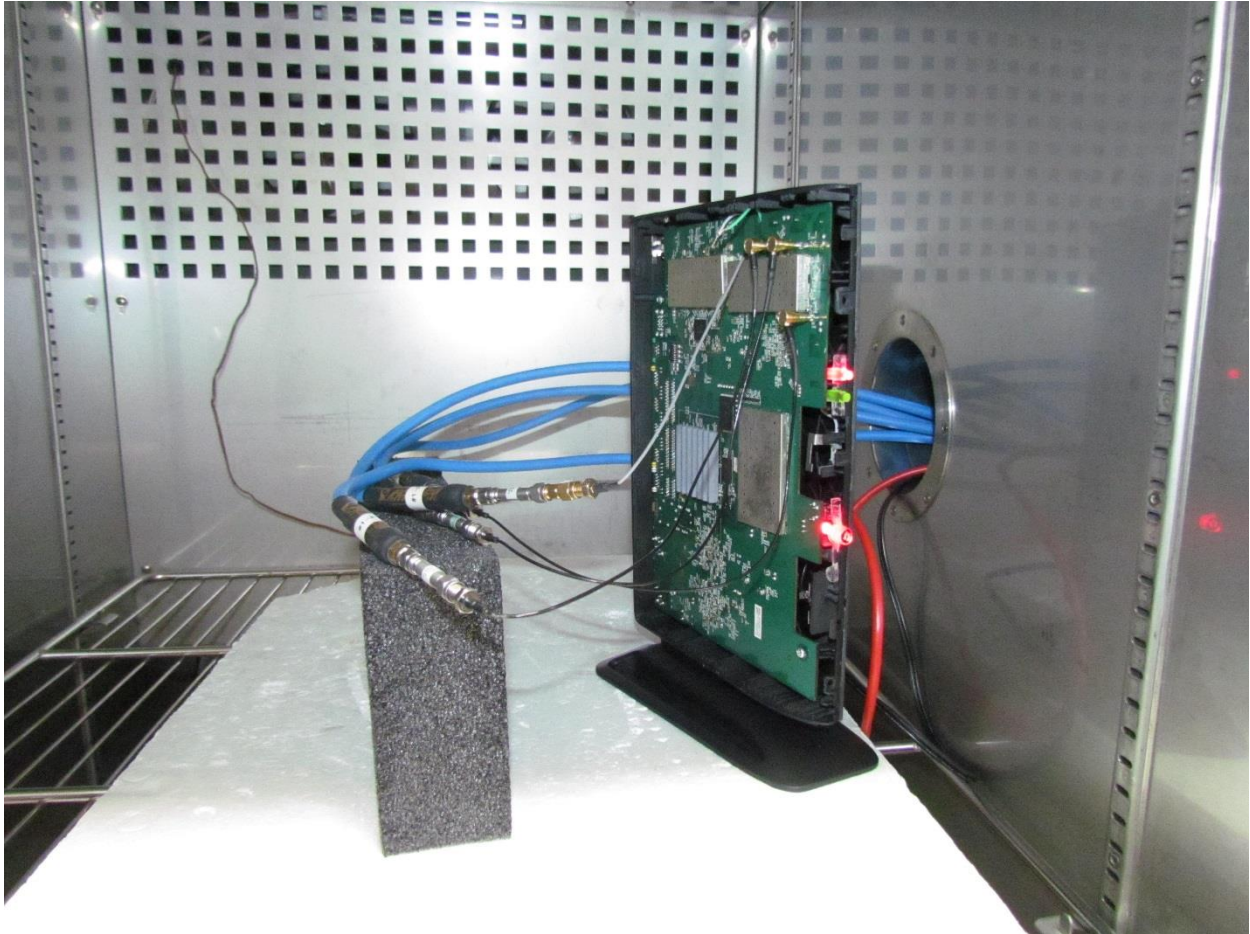
Conducted RF
