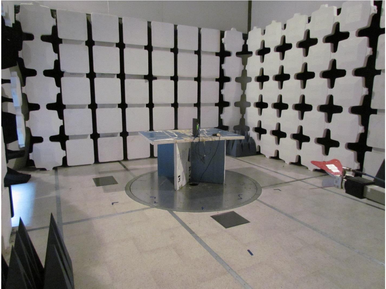
Transmitter Emissions
