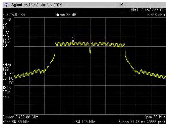
Power Spectral Density Chain 1
