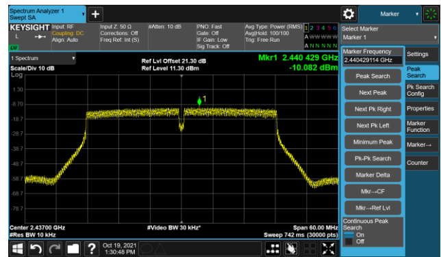
Channel 06 (2437MHz)
