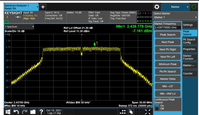
Channel 06 (2437MHz)
