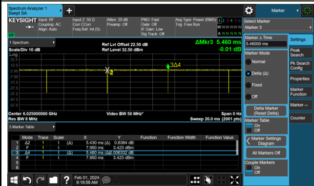
802.11be-EHT40 (T = 5.430ms)
