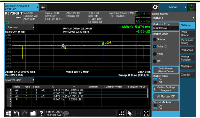
802.11be-EHT320 (T = 5.443ms)
