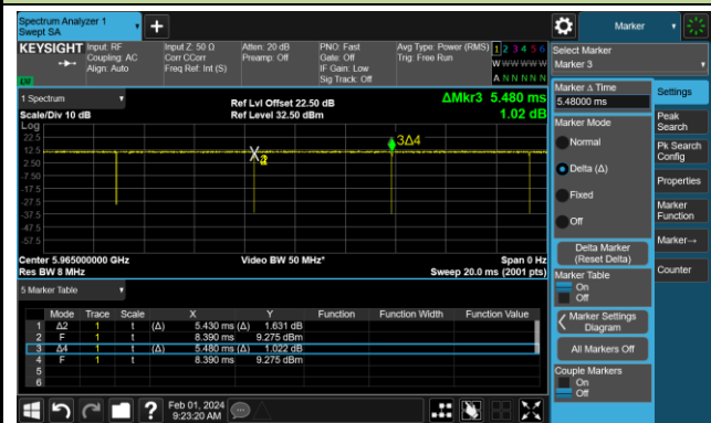
802.11be-EHT160 (T = 5.430ms)
