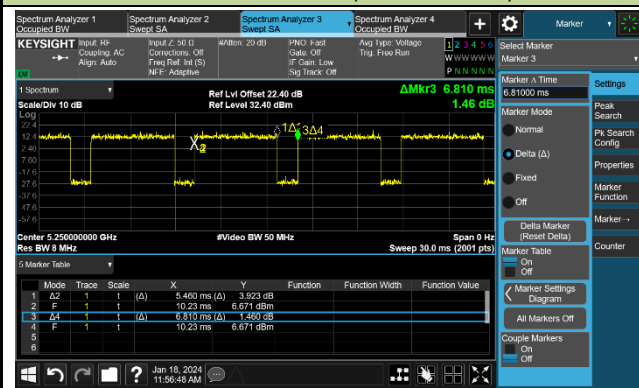
802.11ax-HE160 (T = 5.460ms)
