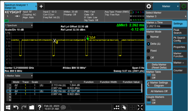
802.11ax-HE80 (T = 2.113ms)
