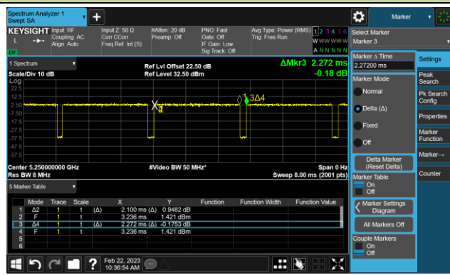
802.11ax-HE160 (T = 2.100ms)
