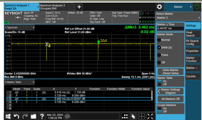
802.11be-EHT40 (T = 5.439ms)
