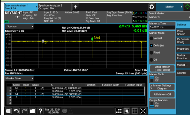
802.11be-EHT20 (T = 5.439ms)
