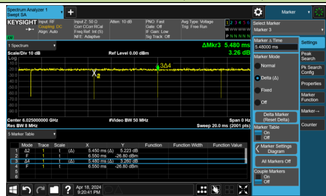
802.11be-EHT160 (T = 5.450ms)
