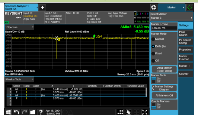
802.11ax-HE80 (T = 5.460ms)
