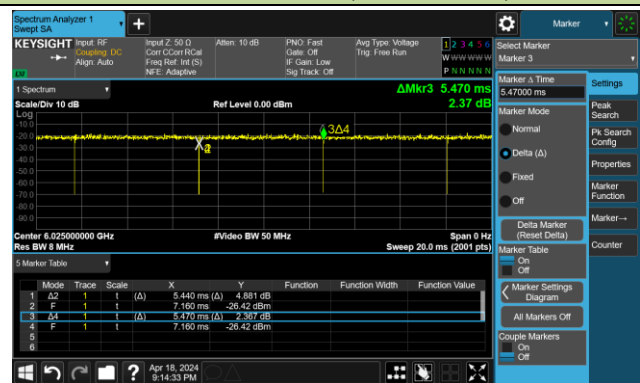
802.11be-EHT40 (T = 5.470ms)
