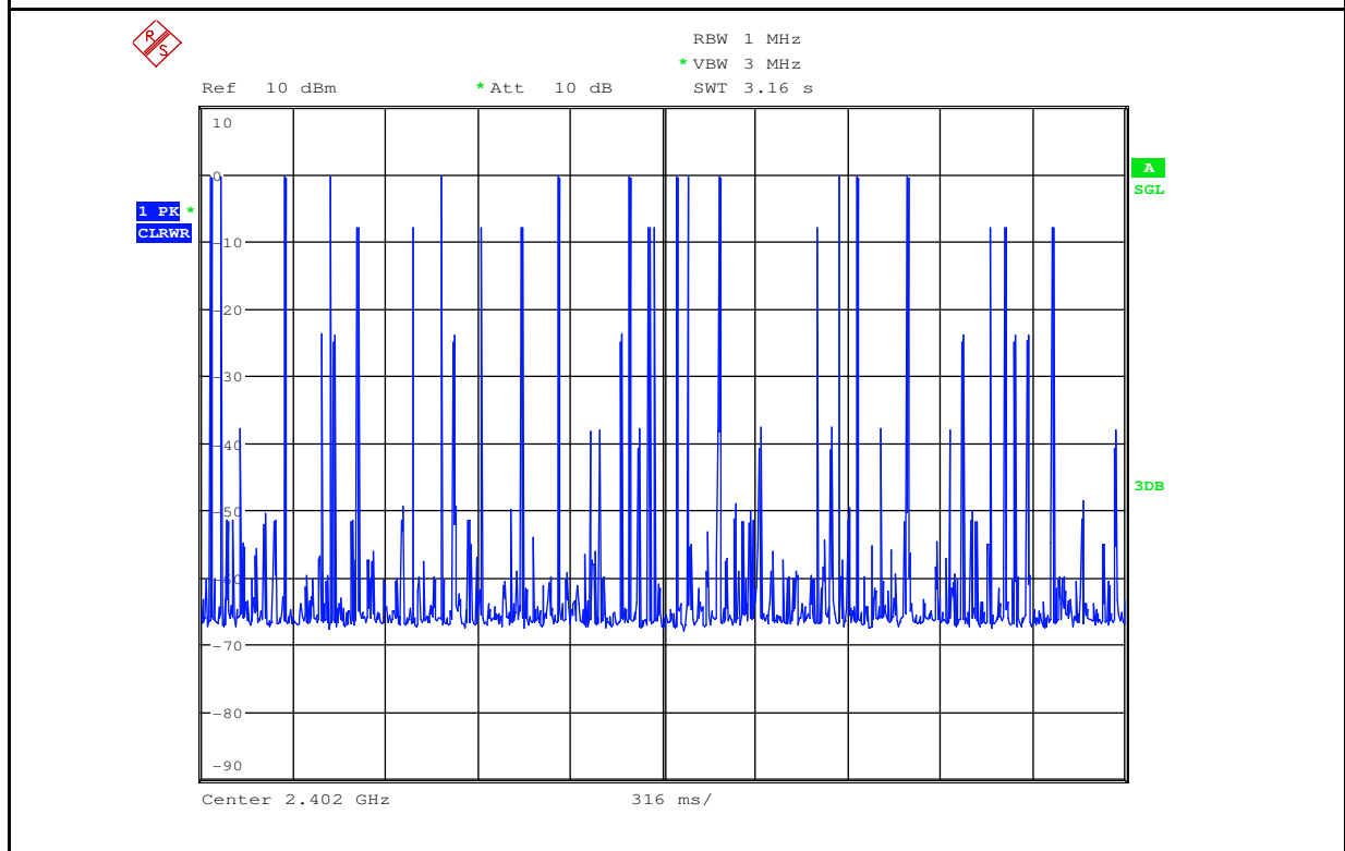
Dwell Time_2DH1_2402
