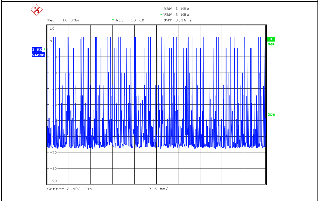
Dwell Time_3DH3_2402
