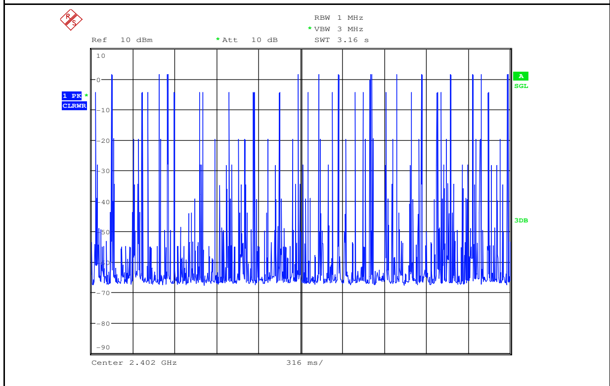
Dwell Time_2DH5_2402
