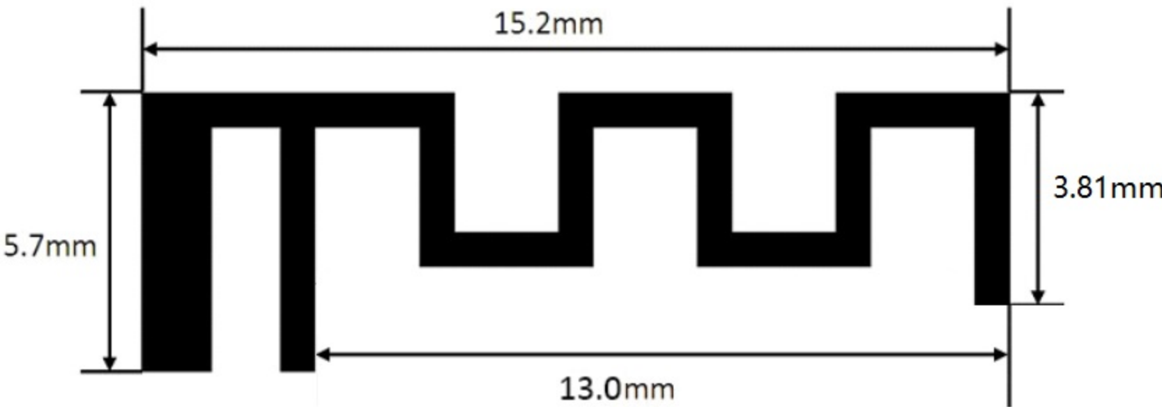
Antenna Photo & Length (mm)
