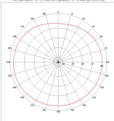
Far-field Power Distribution(H+V) on X-Y Plane Plot Peak Gain(H+V)= 1.25 dB, Plot AvgGain(H+V)= -0.88dB @2.44000 GHz
