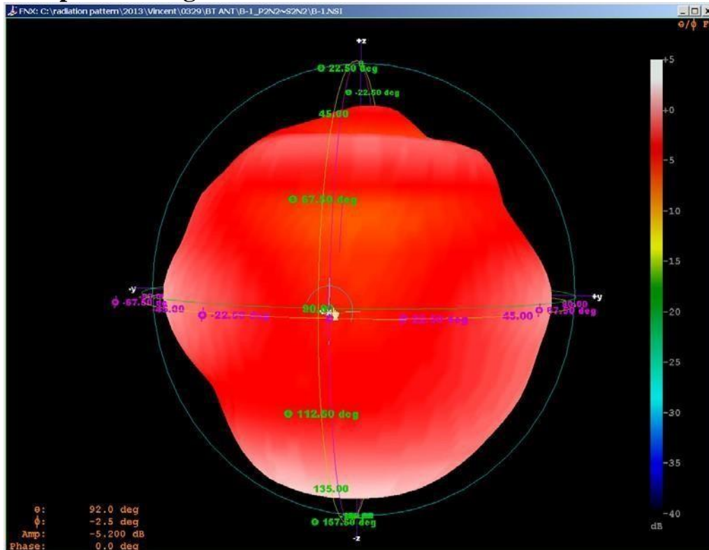
Far-field Power Distribution(H+V) on X-Y Plane Plot Peak Gain(H+V)= 1.25 dB, Plot AvgGain(H+V)= -0.88dB @2.44000 GHz
