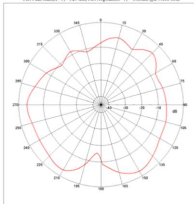
Far-field Power Distribution(H+V) on X-Z Plane Plot Peak Gain(H+V)= 1.25 dB, Plot AvgGain(H+V)= -3.83dB @2.44000 GHz
