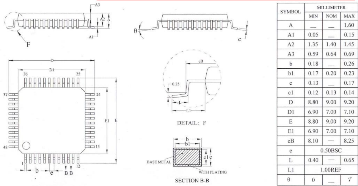
Figure 3-1. AC6921A_LQFP48 Package
