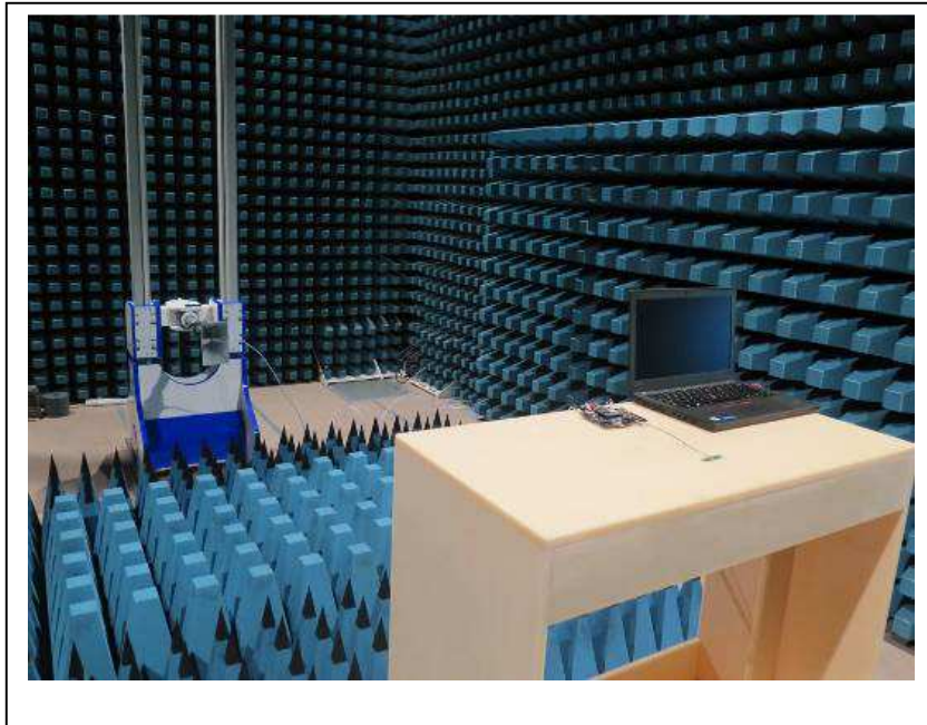
Test setup1 for Wi-Fi
