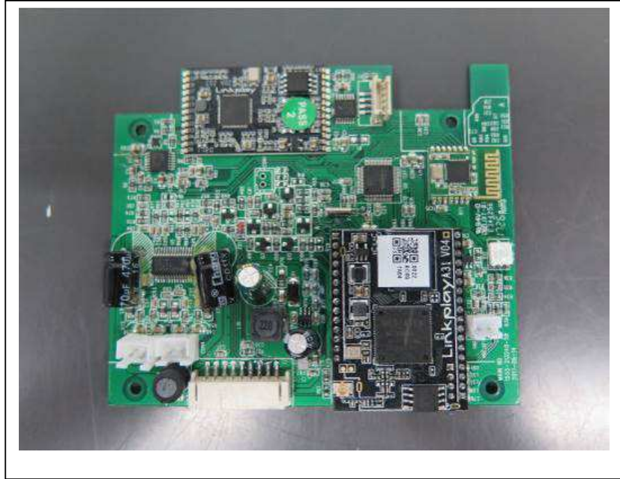
Internal Configuration 1 (Main PCB)
