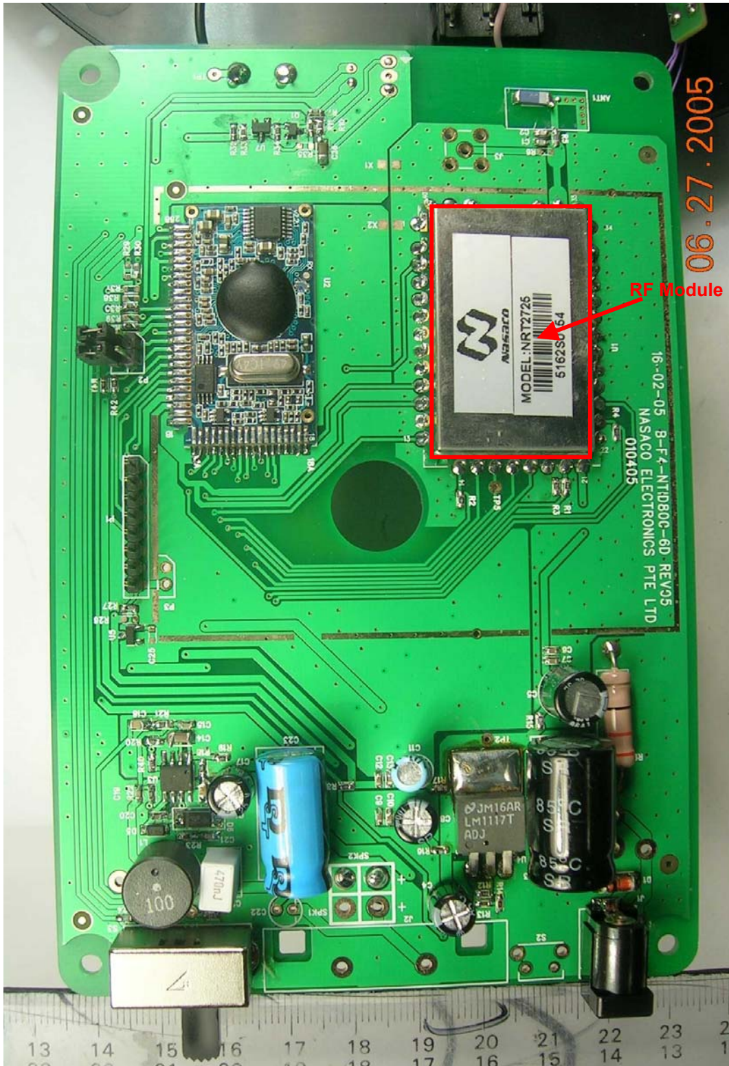
EUT PCB Component Side
