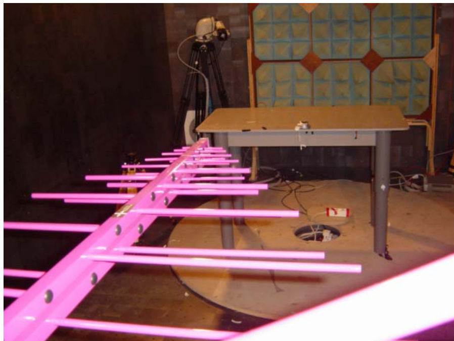
Set-up for Radiation Susceptibility (Reference picture)
