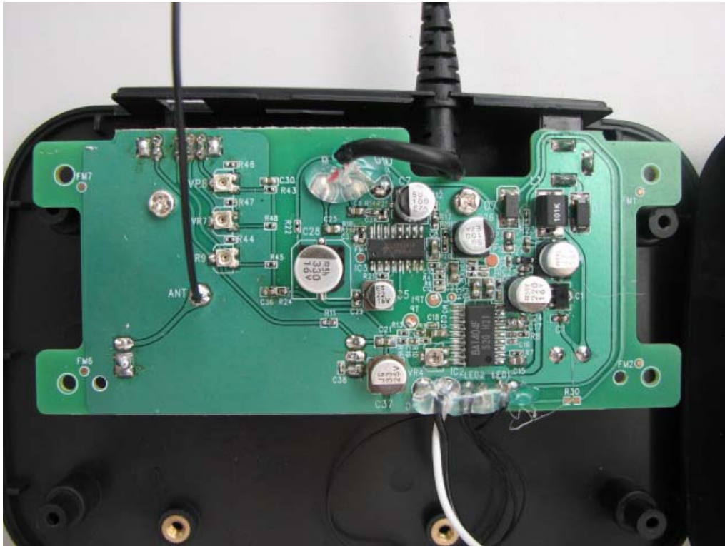
MGJ7140 Transmitter
