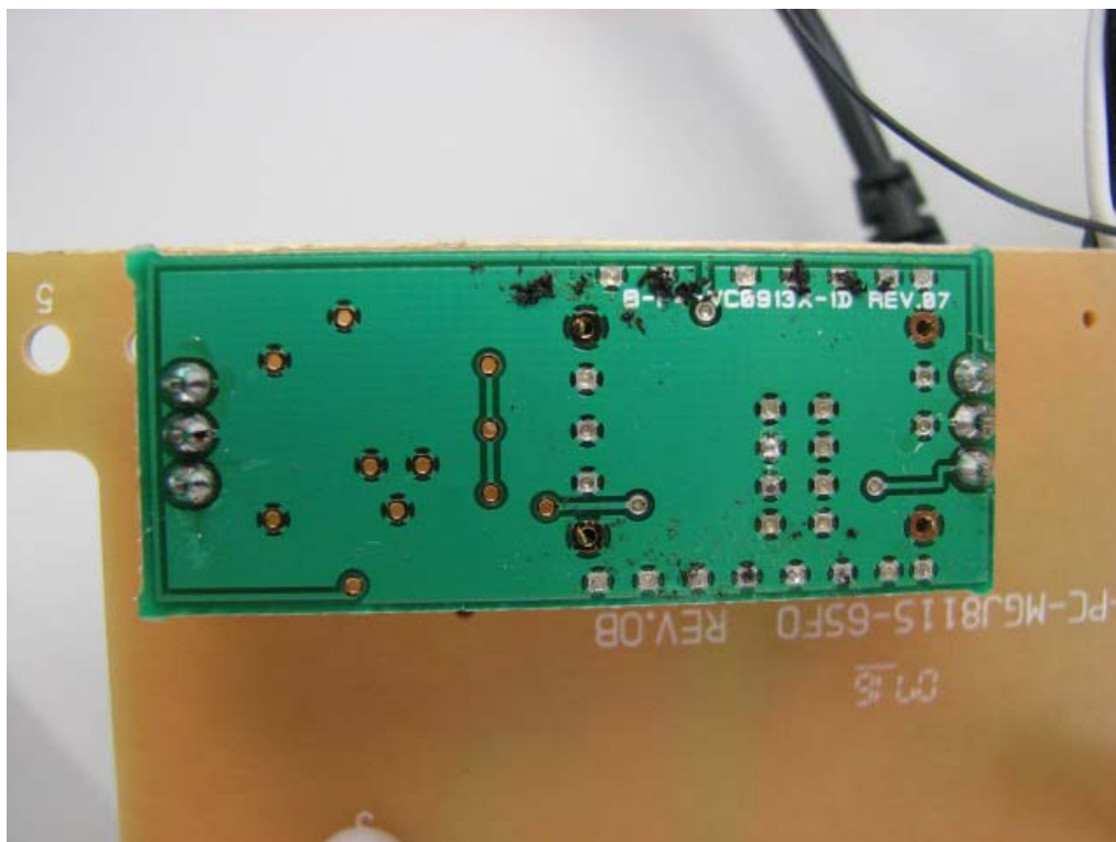
MGJ7140 Transmitter
