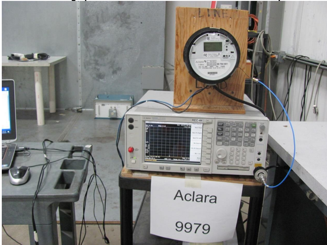
Photograph of Antenna Conducted Emissions Test Setup
