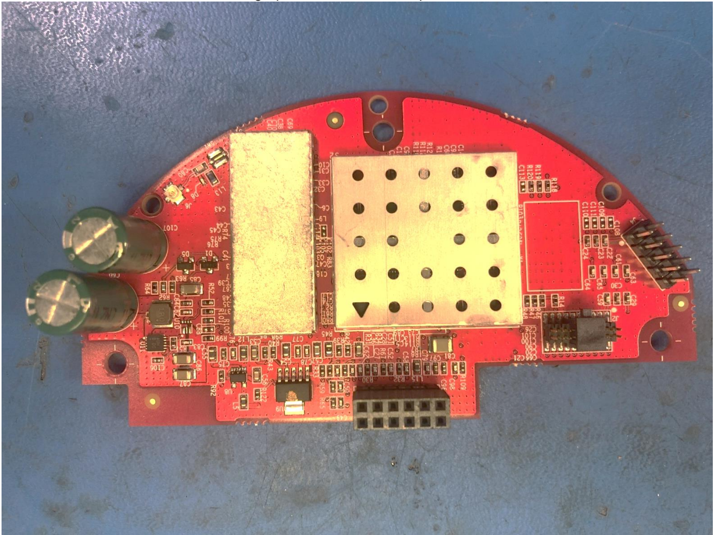
Photograph of PC Board: Component Side
