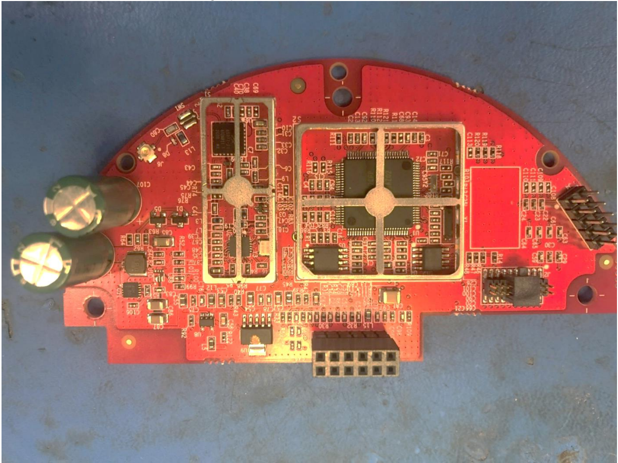
Model: Y84580-2 Photograph of PC Board: Shield Removed
