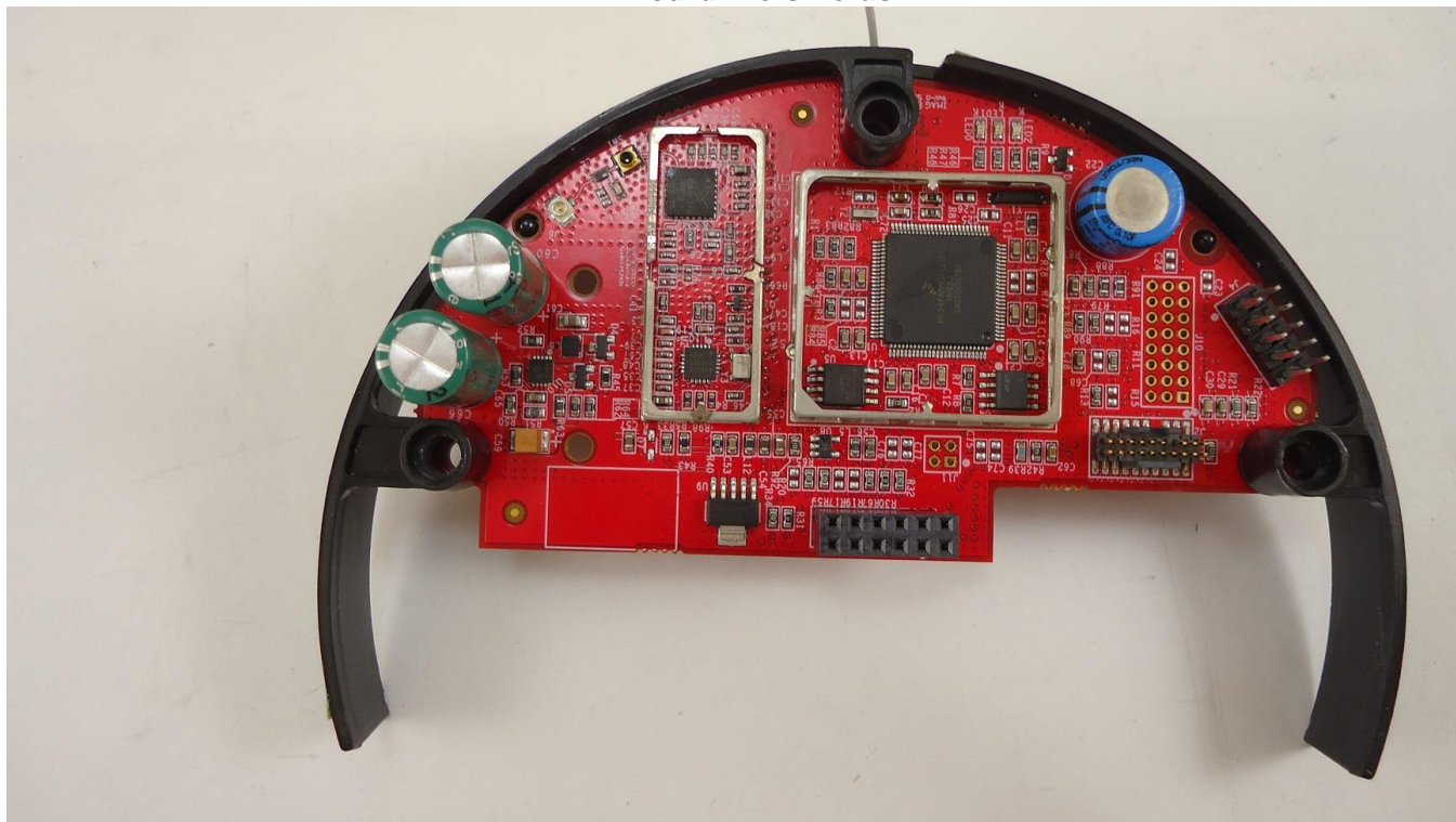
RF Board: no shields
