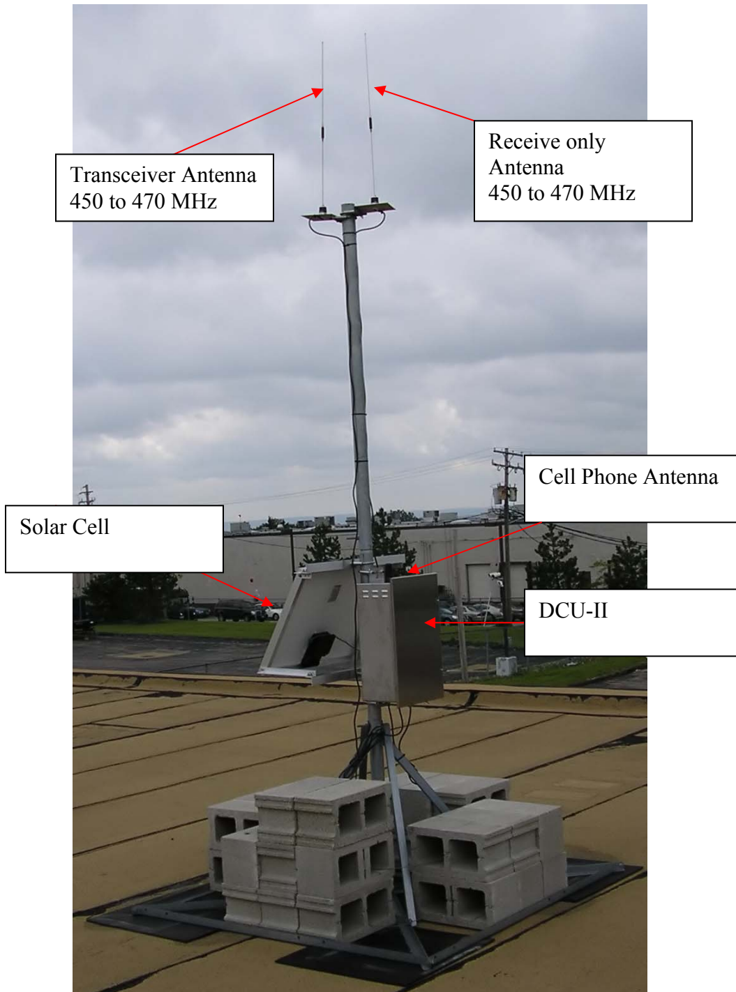
General observation of the roof-mounted LLB9975 Hexagram's DCU-II
