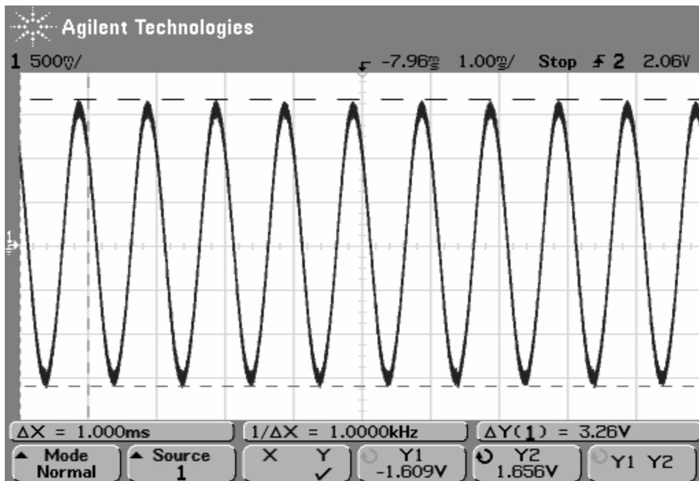
Fig. 3 \pm 12.5 kHz modulated test signal 25 kHz = 3.26 V.
