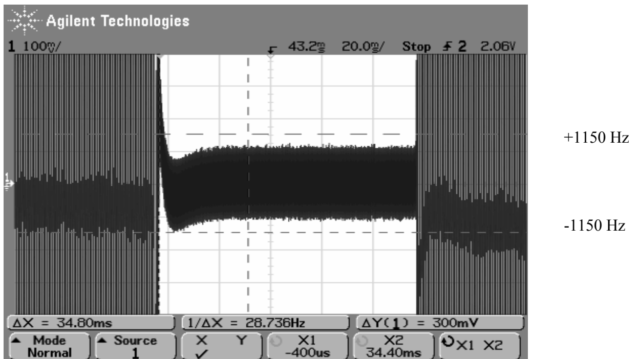
Fig. 5 Full Transmission
