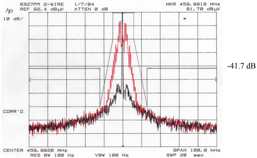
Fig. 1 Hexagram Model 6327PM MTU Emissions Mask
