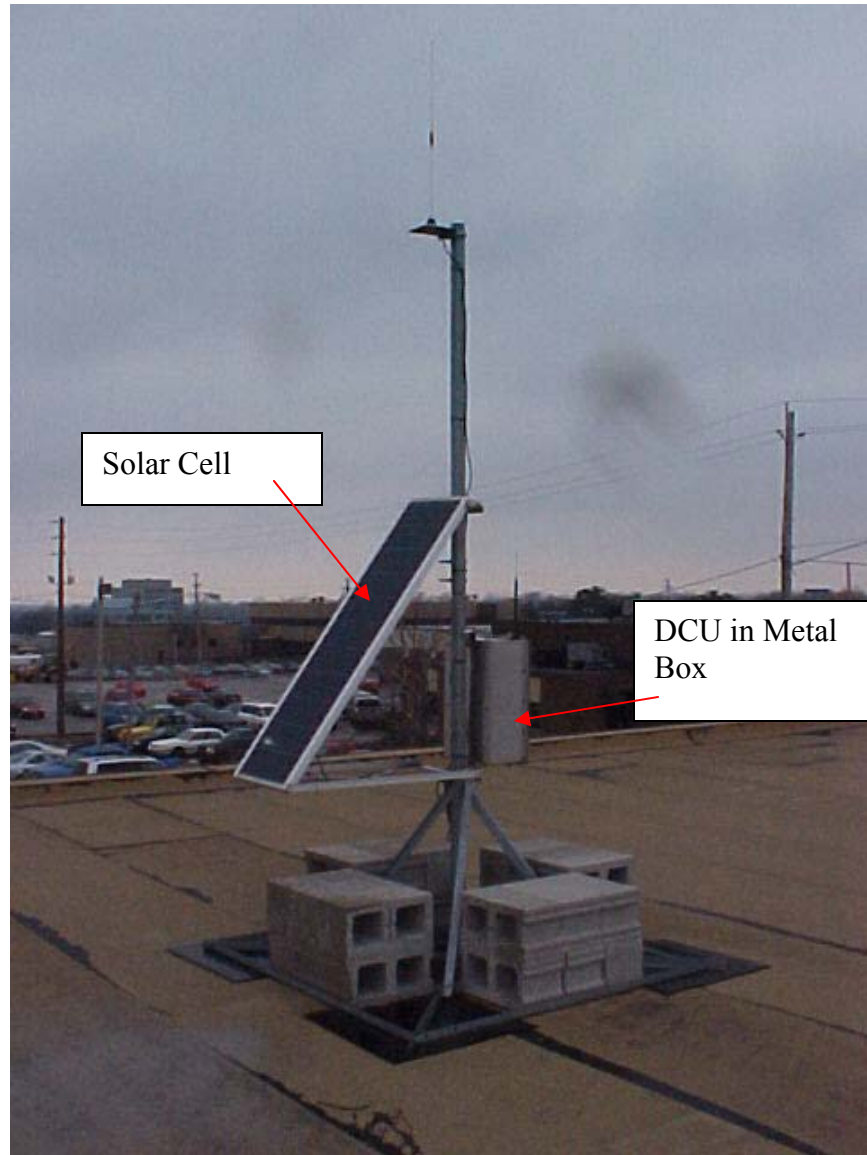
DCU Installed on a roof
