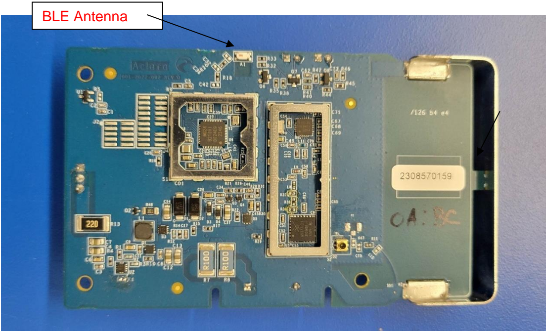
Photograph of PC Board: Component Side with shields removed
