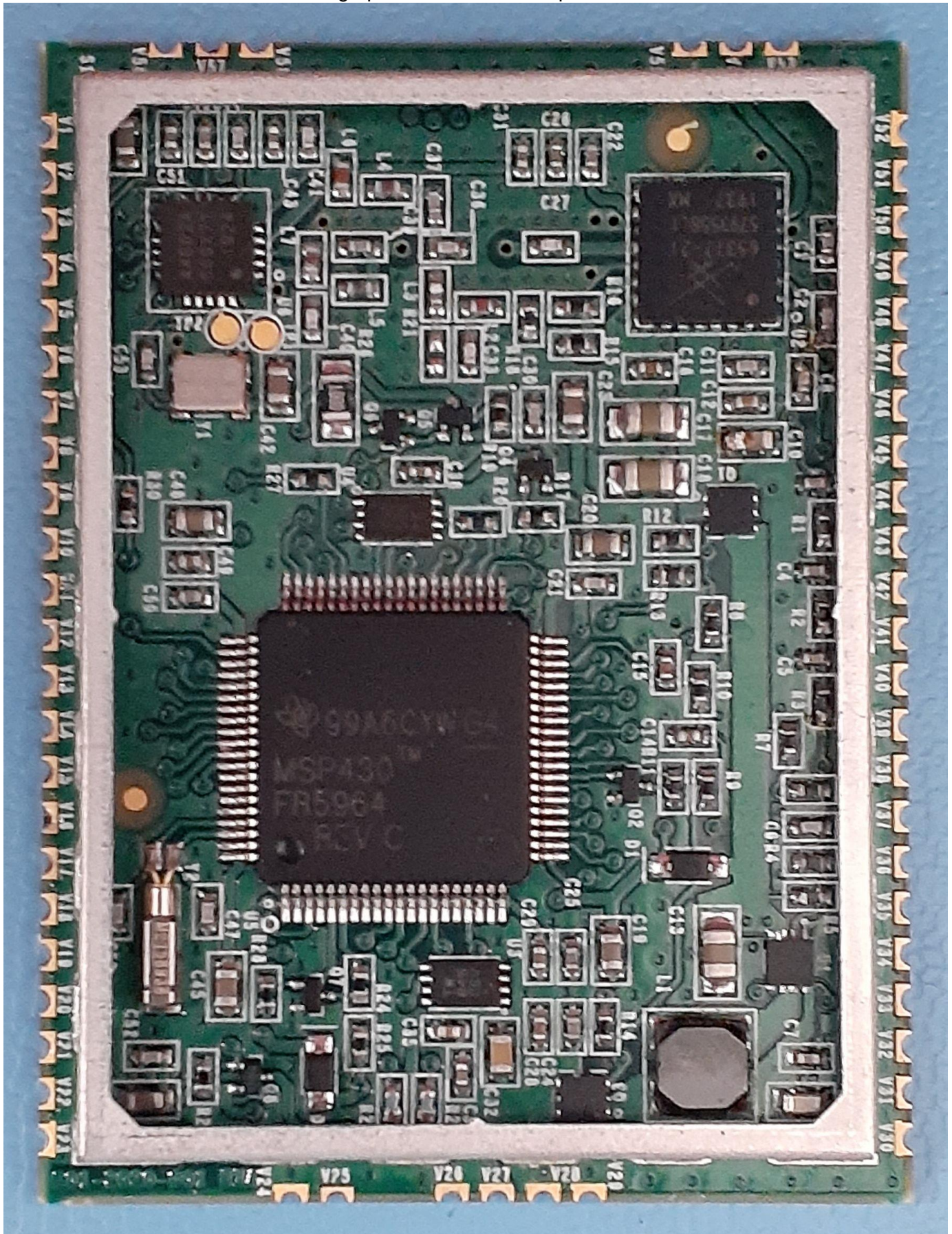
Photograph of PC Board: Component Side
