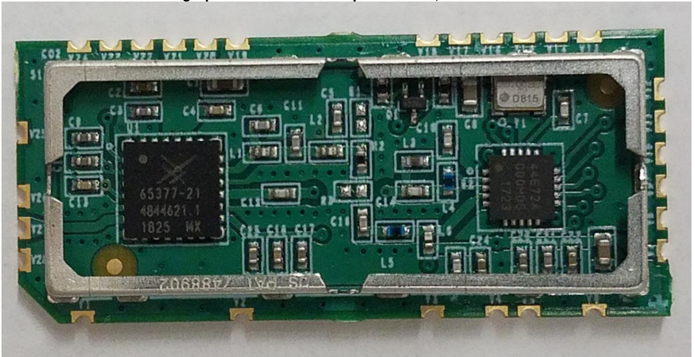
Photograph of RF Board: Component side, Shield removed
