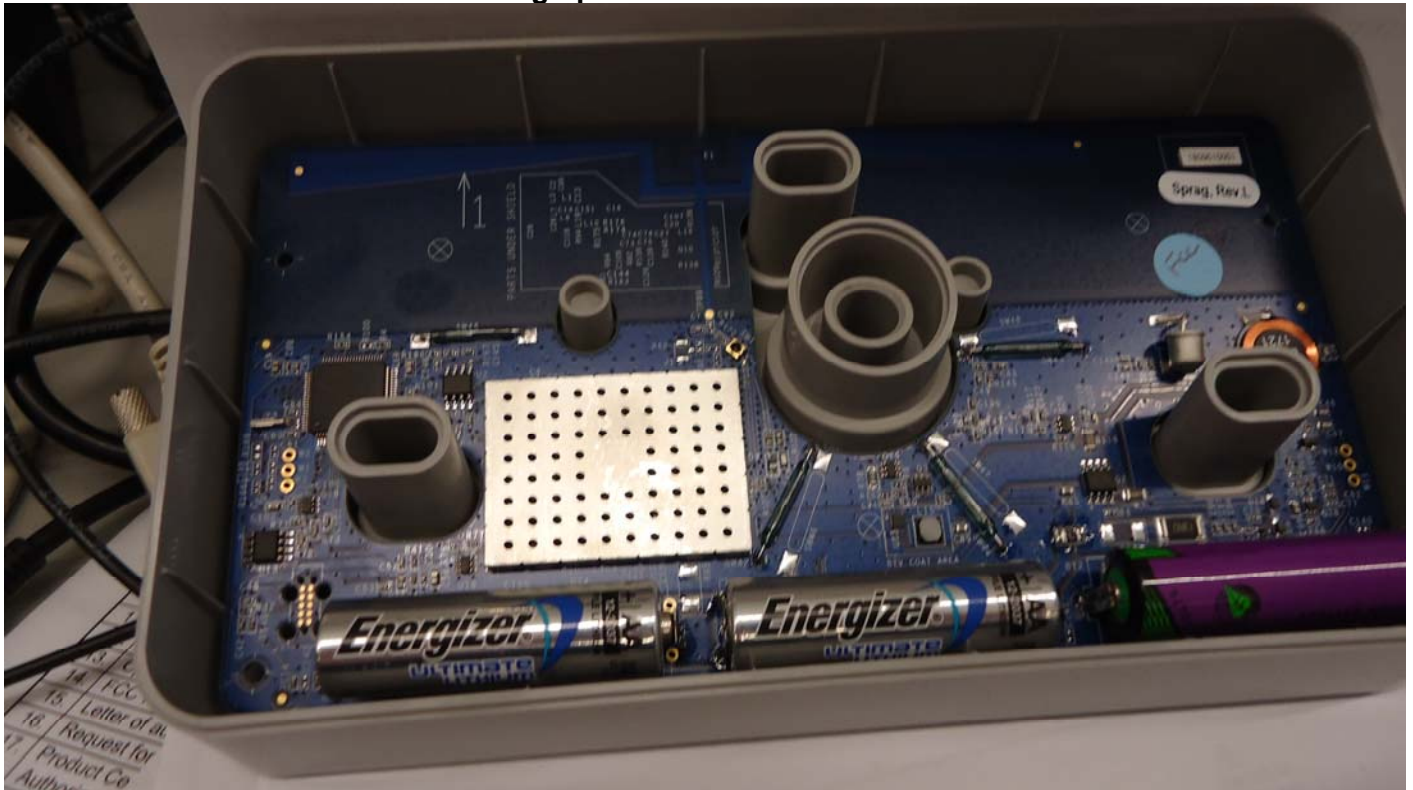
Photograph of PCB inside Enclosure
