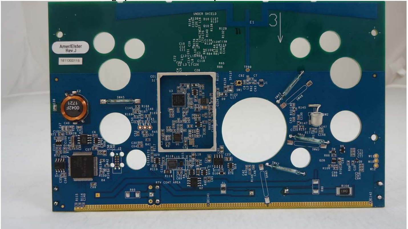
Photographs of PC Board: Component side without shield
