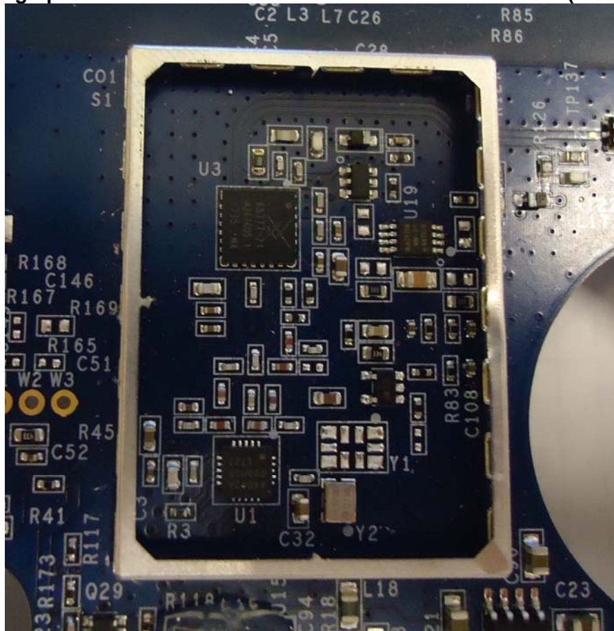
Photographs of PC Board: Radio Section with Shield Removed (Close Up)
