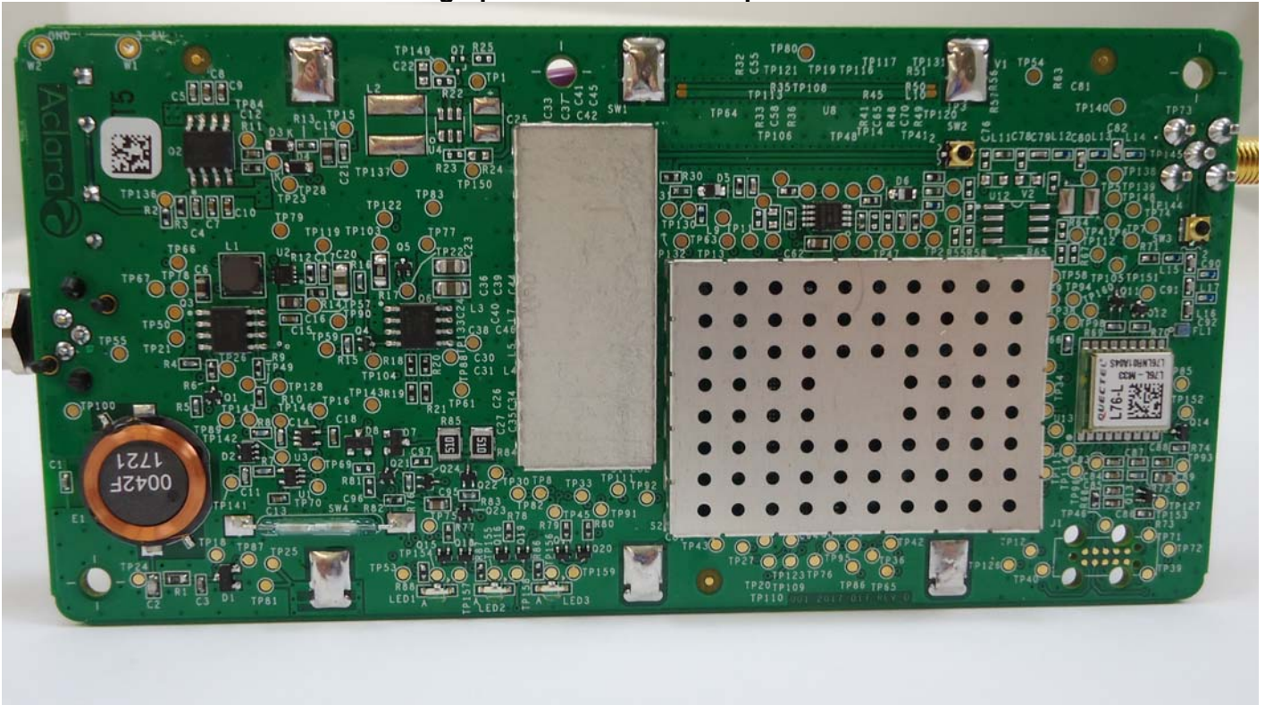
Photograph of PC Board: Component Side
