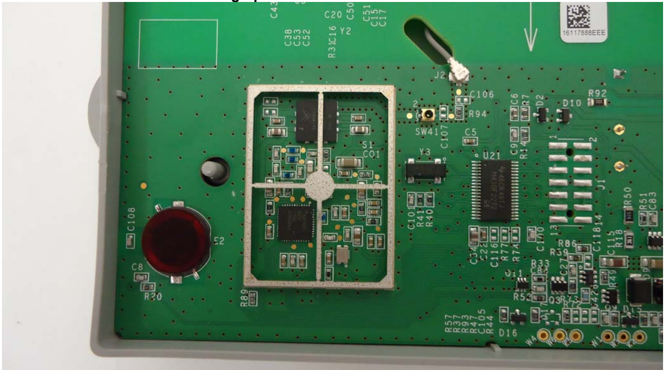
Photograph of PC Board: Shield removed
