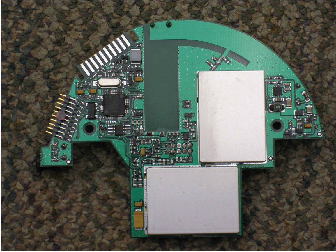
Components layer with shields
