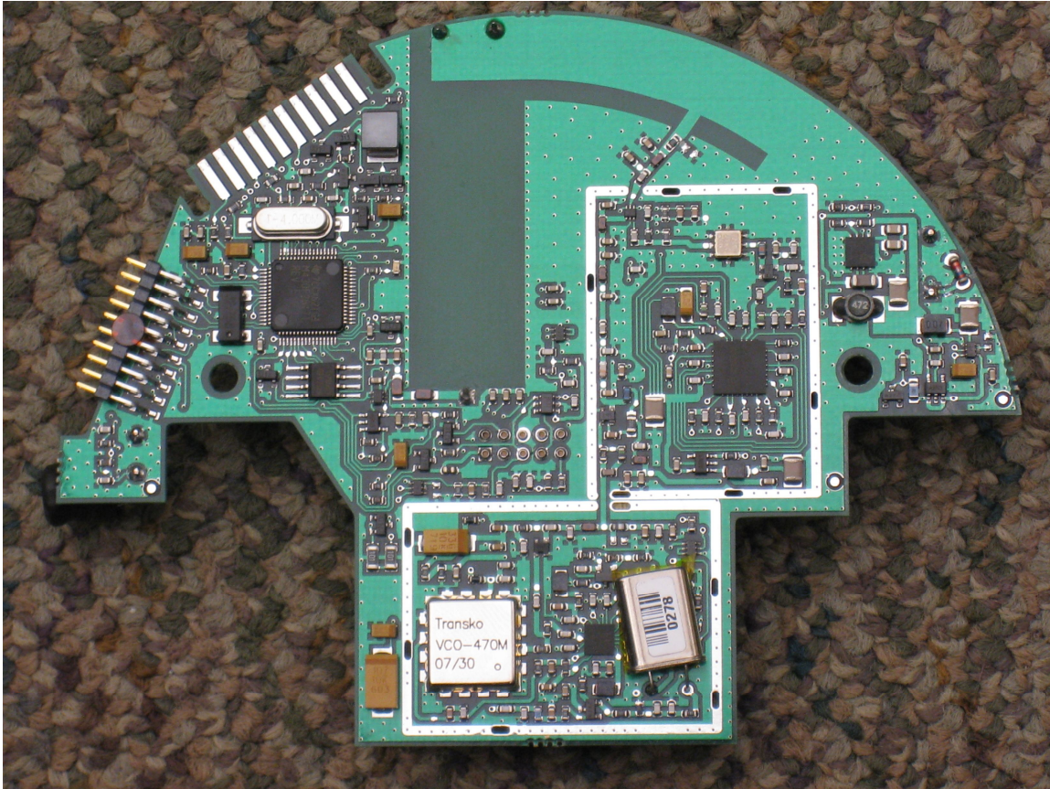
Components layer with no shields
