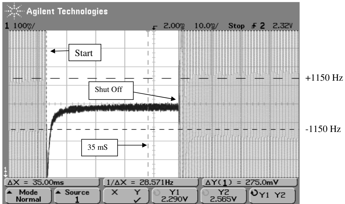
Fig. 5 Full Transmission
