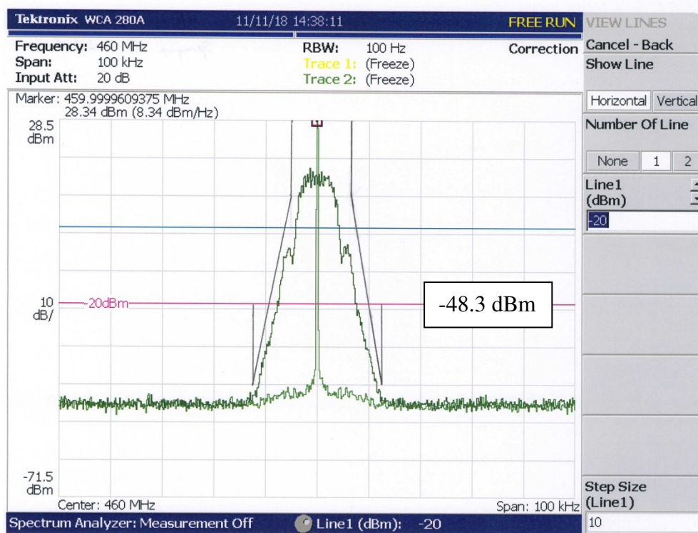
Fig. 1 Hexagram Model 2011-009X Emissions Mask
